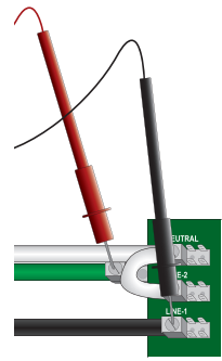
Line-1 and Ground 120VAC (108VAC-132VAC)
